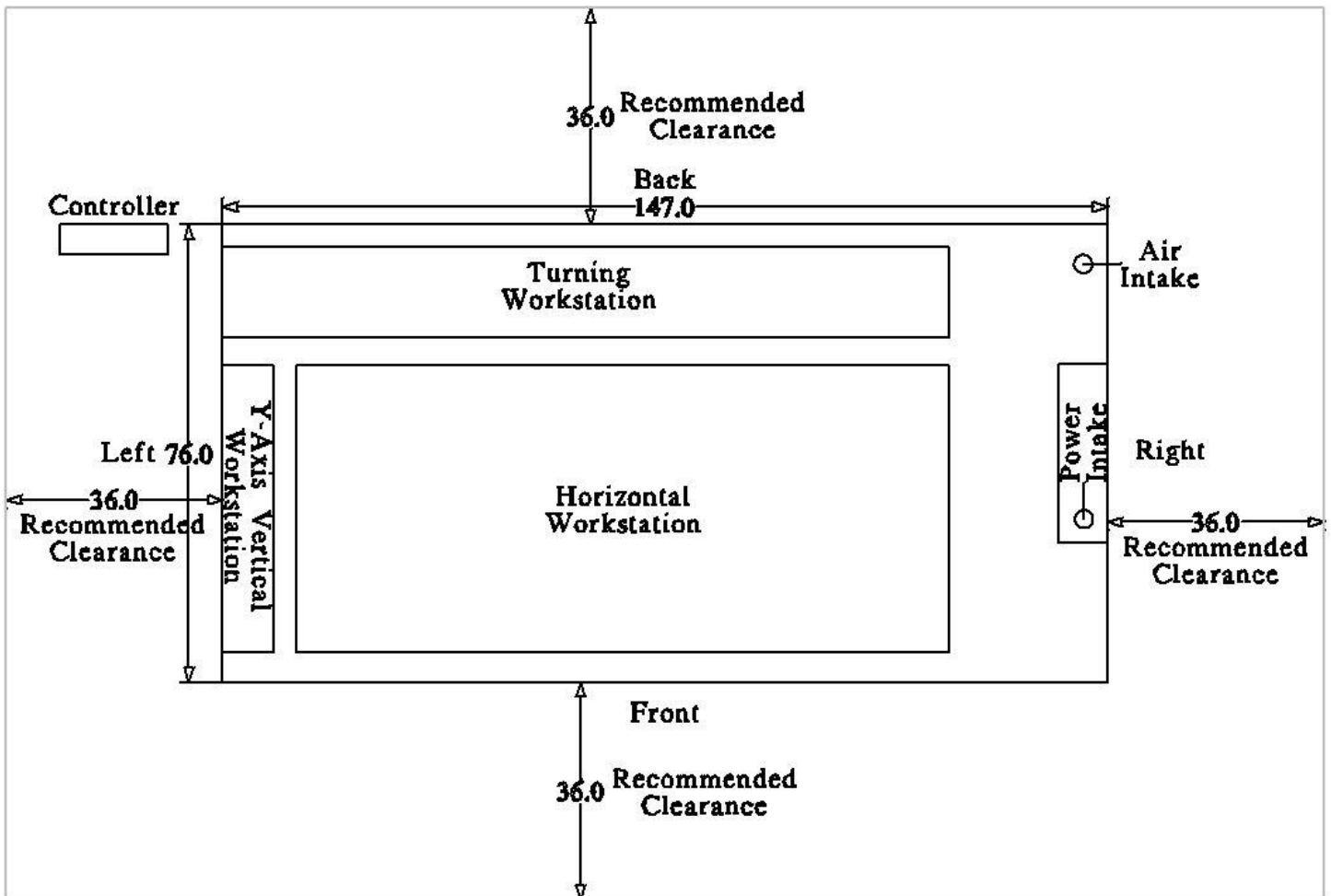
Maverick 4x8 Top View Floor Plan
